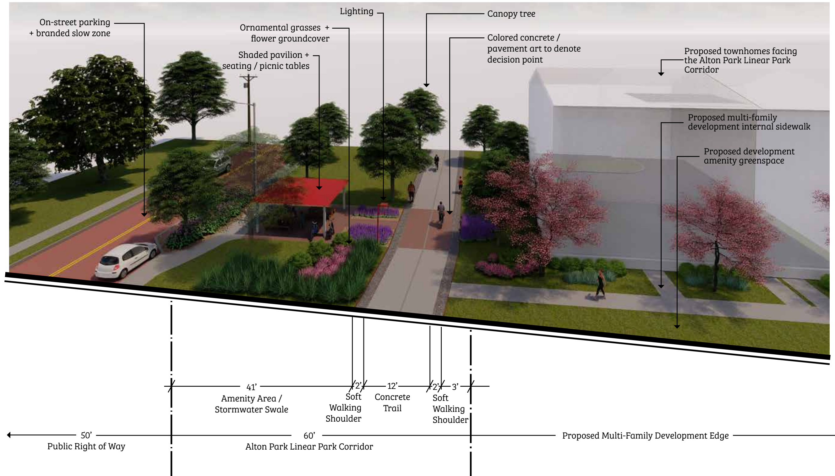
Figure 2.16 - Proposed At Grade/Depressed Trail with a Public ROW Edge and Proposed Multi-Family Development Edge
