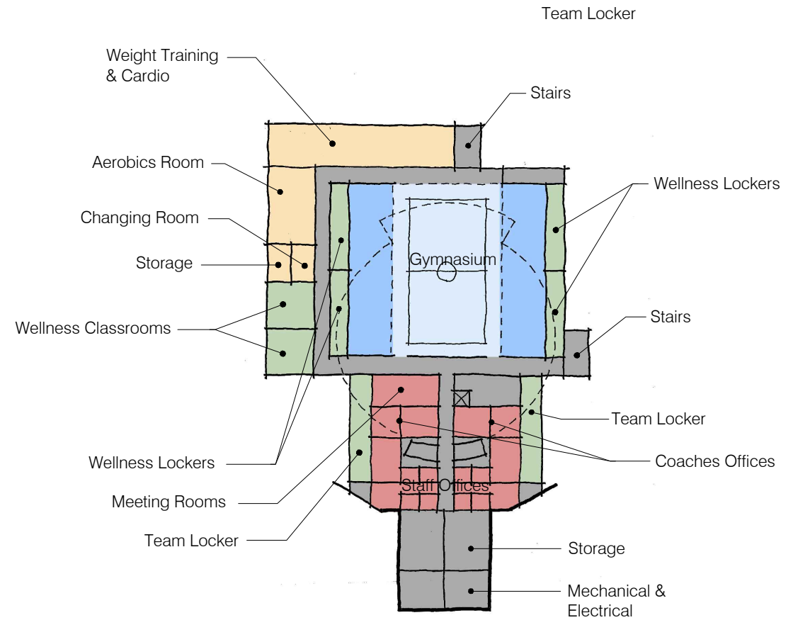
LOWER LEVEL PLAN DIAGRAM 36,825 S.F.
