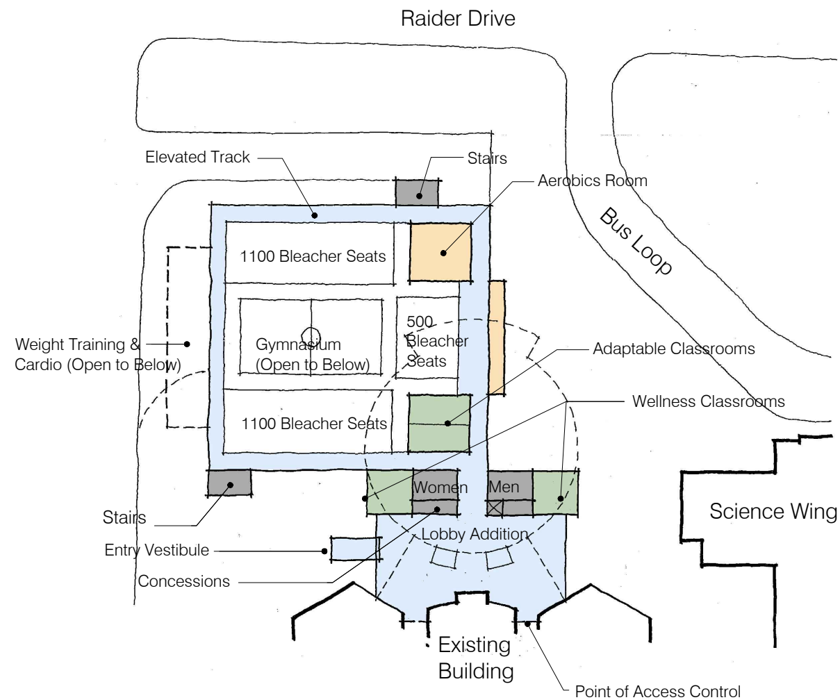
UPPER LEVEL PLAN DIAGRAM 22,035 S.F.
