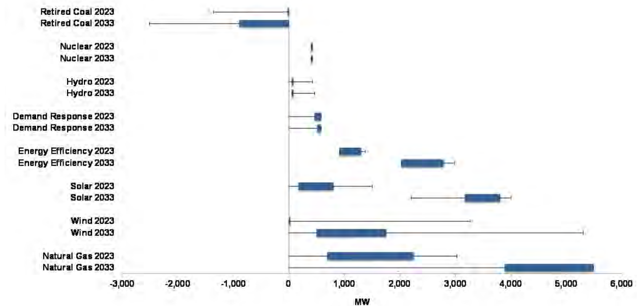
Figure 6-10 Range of resource additions by 2023 and 2033 in the recommended Target Power Supply mix.
