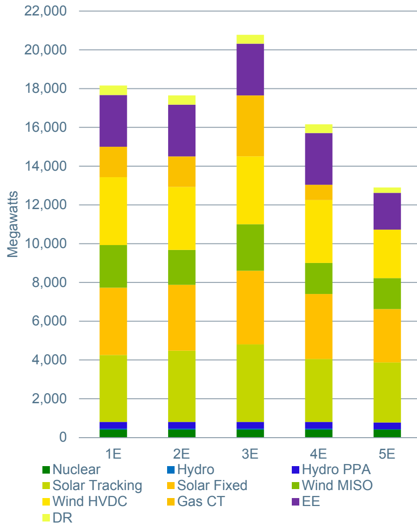
Figure 9 Strategy E capacity additions through 2033 by resource type for the five scenarios.
