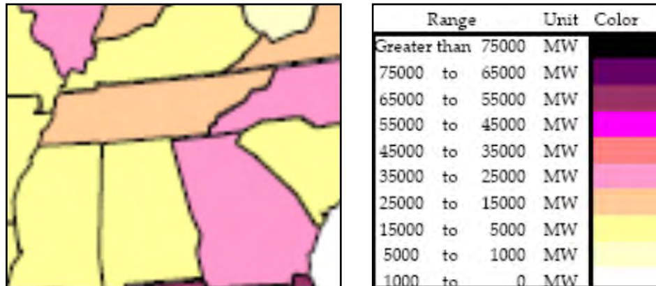
Figure 4-38 Rooftop PV technical potential for states in the TVA region. Source: Adapted from Paidipati et al. (2008).
