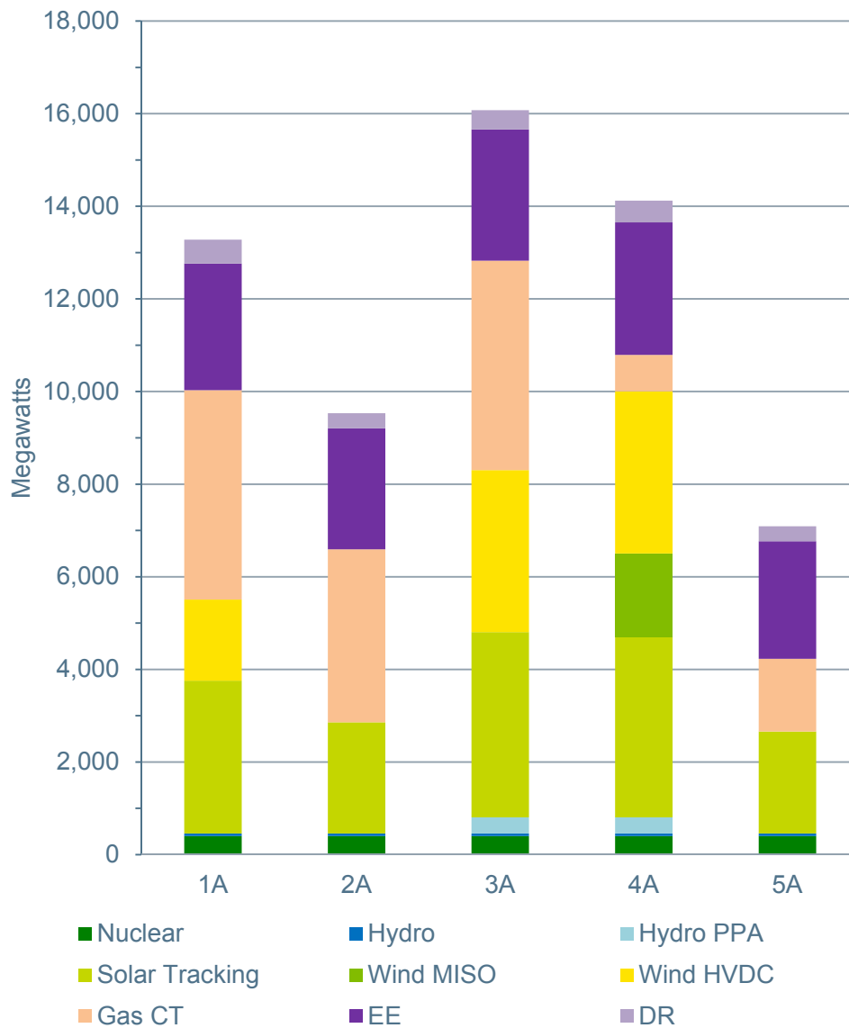
Figure 5 Strategy A capacity additions through 2033 by resource type for the five scenarios.
